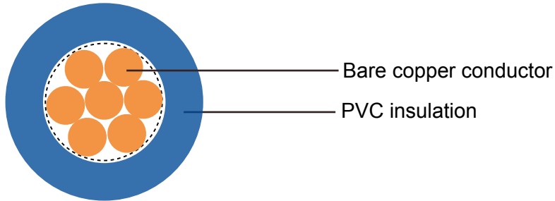
H05V-R
